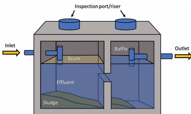
Figure 1: Illustration of a septic tank. Fats, oils, and grease that make up the scum layer float on the top, while heavier solids that make up the sludge settle to the bottom. This allows effluent water to leave the tank and enter the drainfield where it is treated by the soil.
