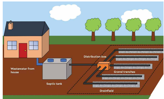
Figure 2: Effluent leaves the septic tank and is distributed through the drainfield via a distribution box. Effluent is treated as it passes through the soil profile.
